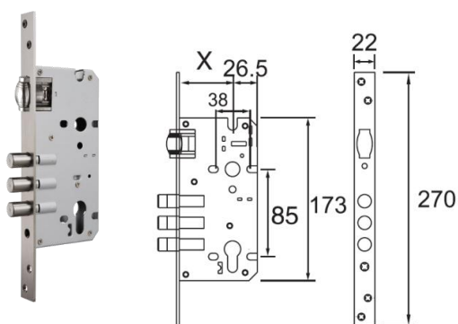
X: 50/60mm Multiple Point Roller
