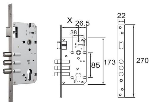
X: 50/60mm Multiple Point Entrance
